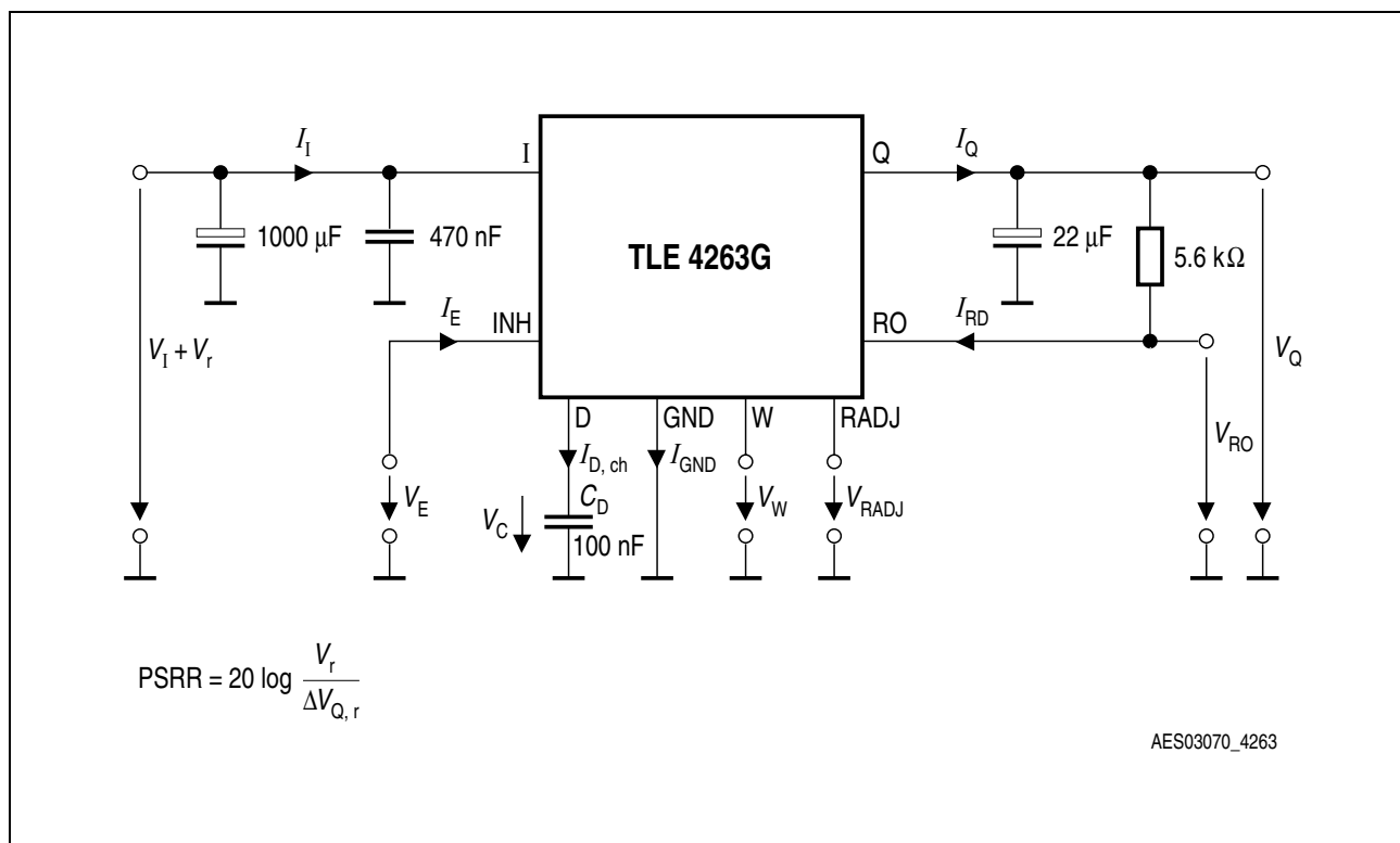
Figure 4 Test Circuit
