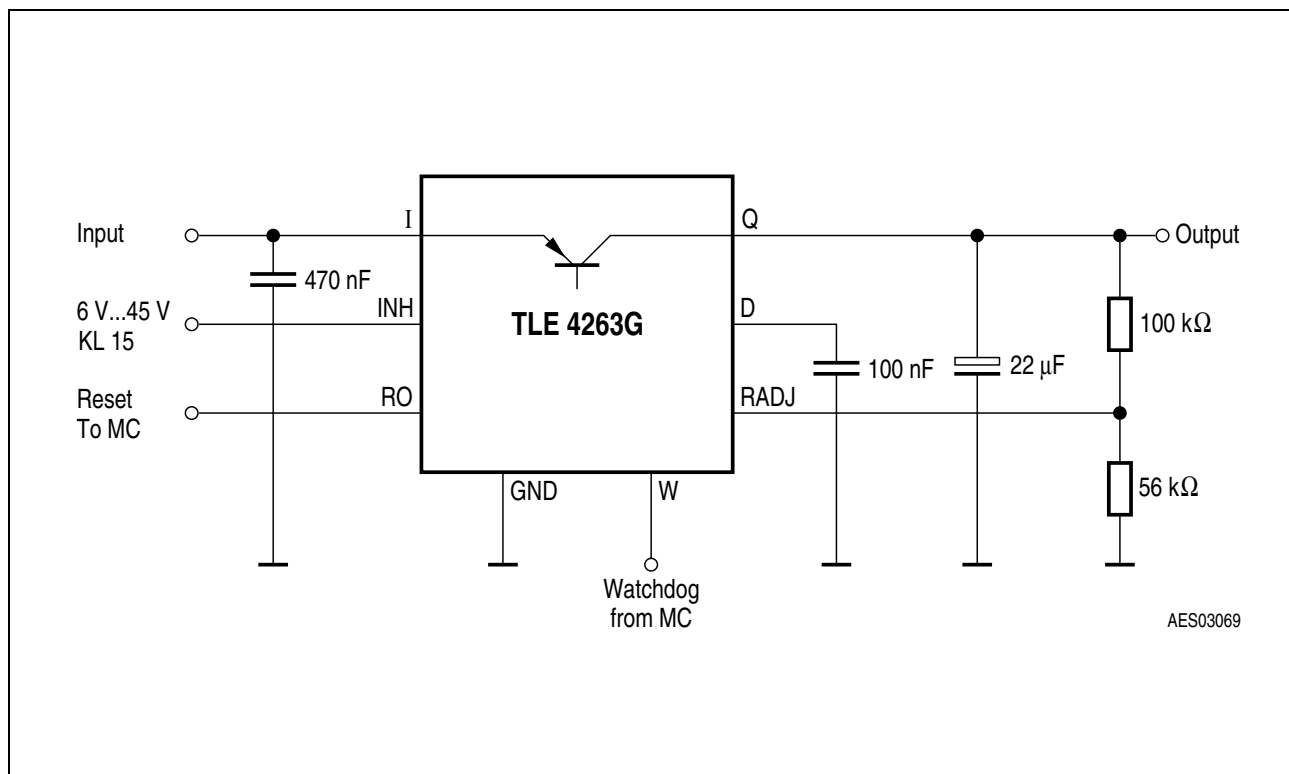
Figure 3 Application Circuit
